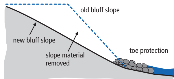
Figure 8: Cutback Slope Stabilization Method
