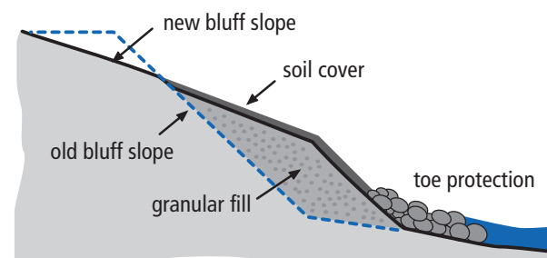
Figure 9: Cut and Fill Slope Stabilization Method
