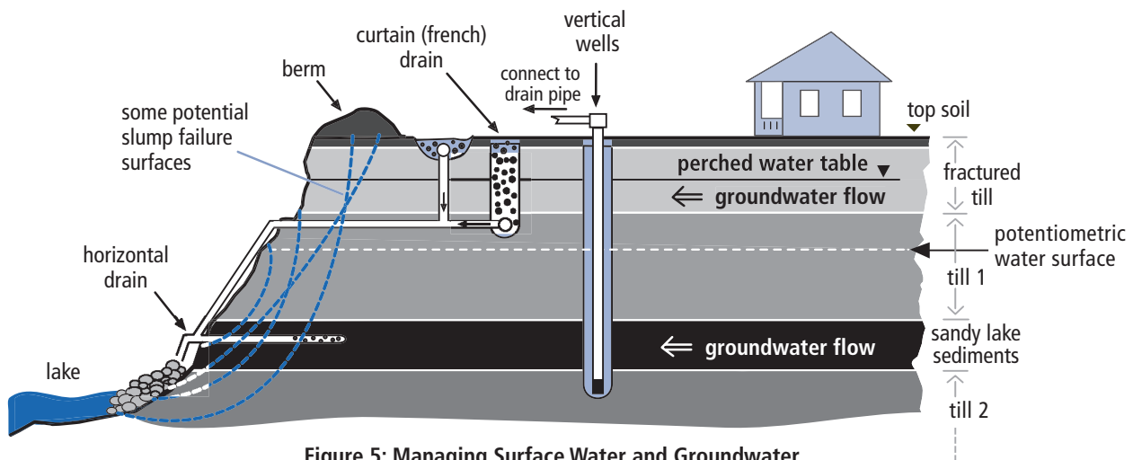
Figure 5: Managing Surface Water and Groundwater
