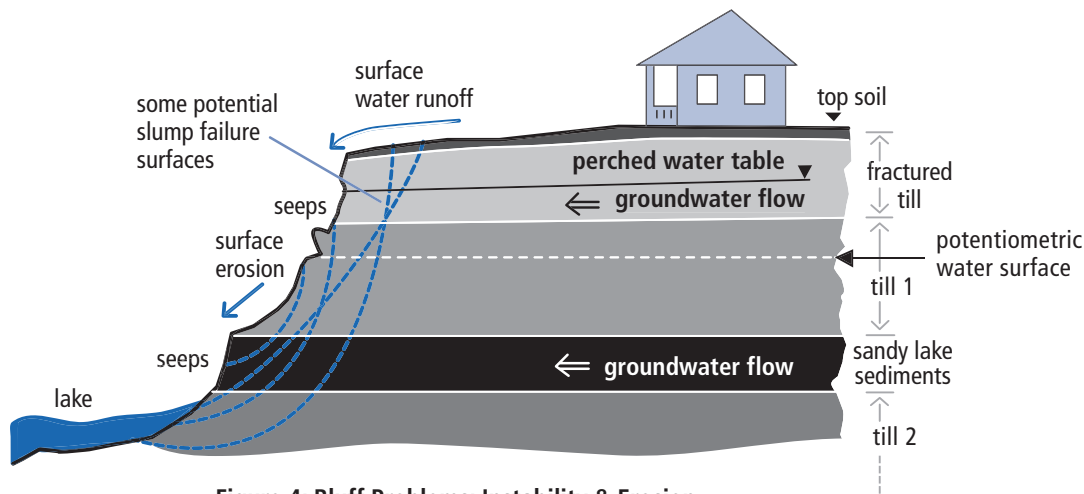
Figure 4: Bluff Problems: Instability & Erosion Surface Water Runoff Groundwater Seepage
